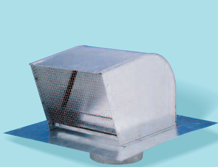
RC Roof Caps For 4, 6 or 8" round duct. 4" duct (Aluminum) 6" or 8" duct (Galvanized Steel). Includes bird screen.
