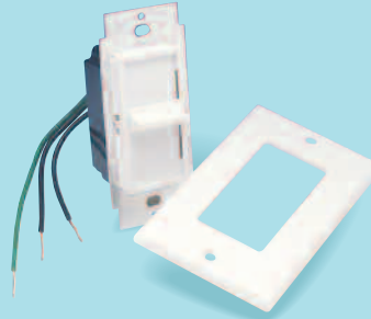
SCD5 Slide Speed Control Decora style slide control with on/off. 115 V/5A
