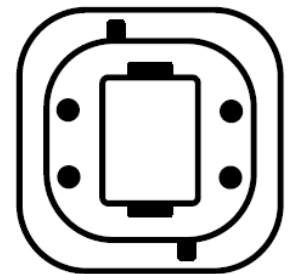
G24q-2 base, 4-pin
